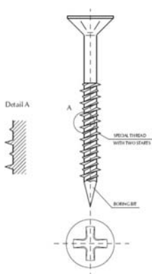
Picture 22. Screw with crossed cutting and double threads
