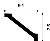
WT2 WALLSTYL®
