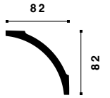
B8 NOMASTYL® 82 x 82 x 2000 mm
