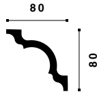
GO NOMASTYL® 80 x 80 x 2000 mm
