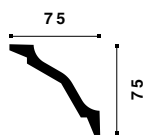
WT26 WALLSTYL®
