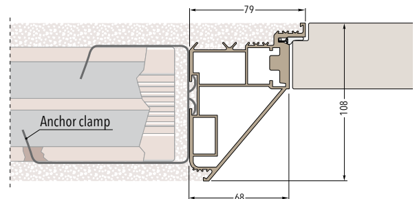
Frame on solid wall - Finished wall thickness 108 mm
