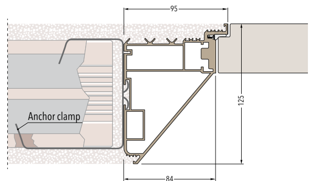
Frame on solid wall - Finished wall thickness 125 mm
