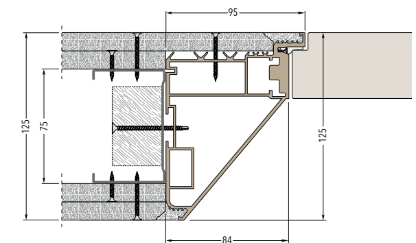
Frame on stud wall with two plasterboards - Finished wall thickness 125 mm
